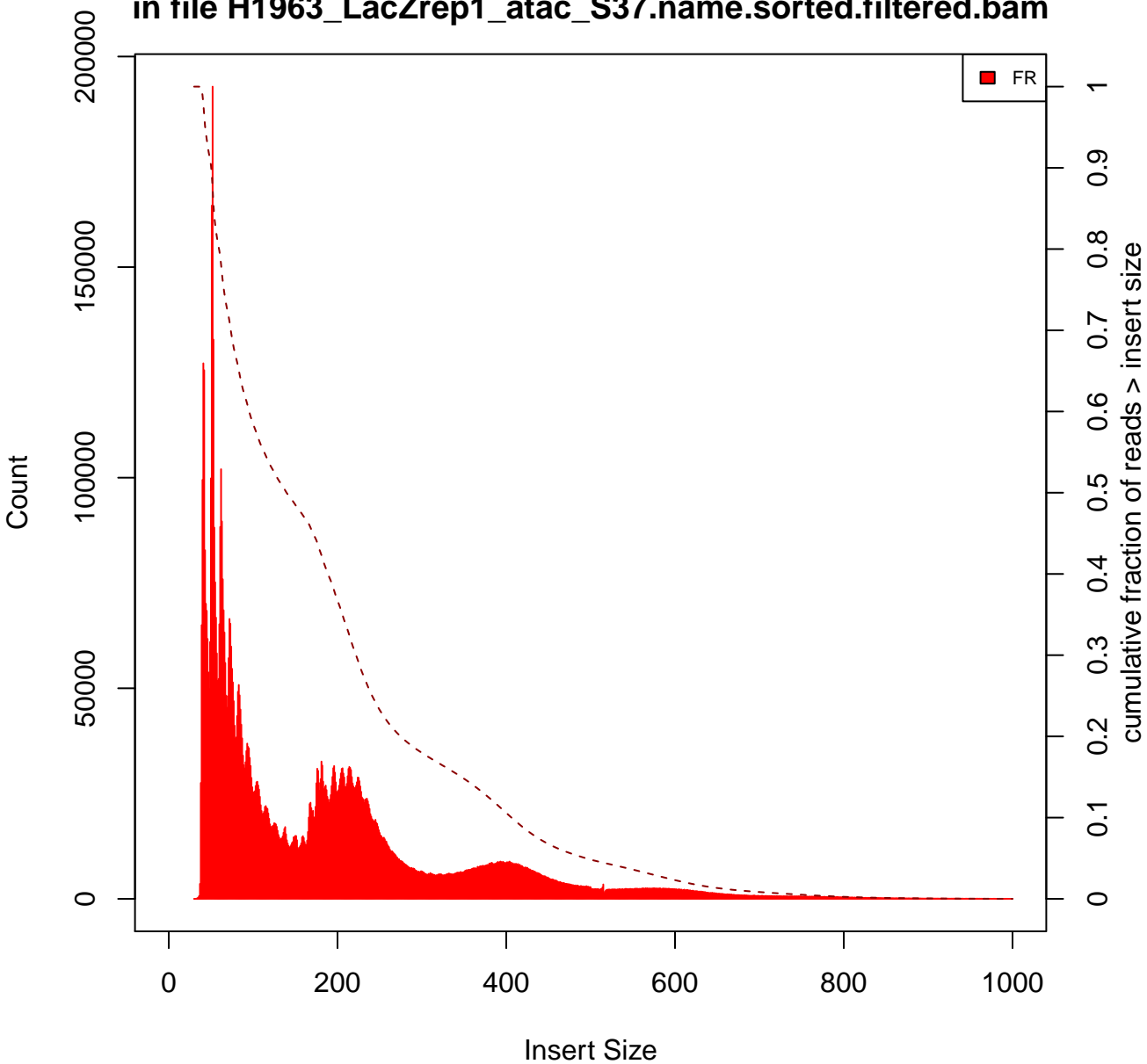
Insert Size Histogram for All_Reads in file H1963_LacZrep1_atac_S37.name.sorted.filtered.bam
