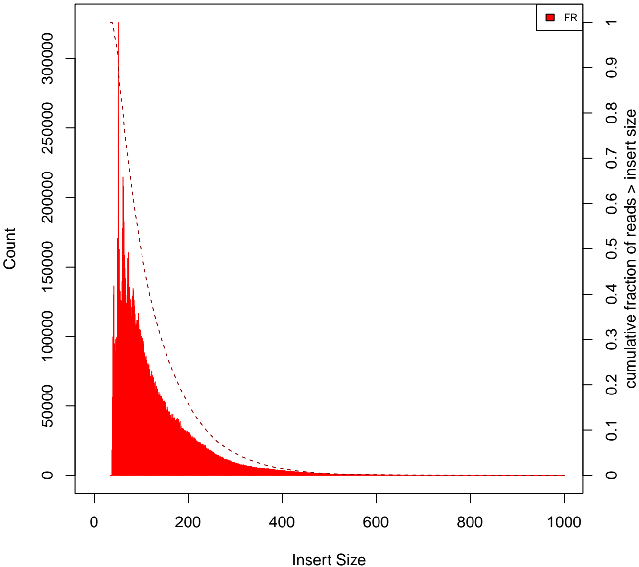
Insert Size Histogram for All_Reads in file H82_ATAC_S2.name.sorted.bam
